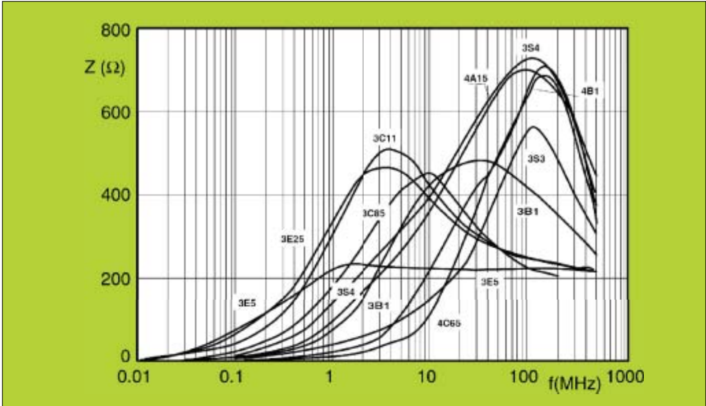
Fig. 3 Impedance versus frequency for several ferrite materials. ( measured on TN12.5/7.5/5 ring cores with 5 turns )
