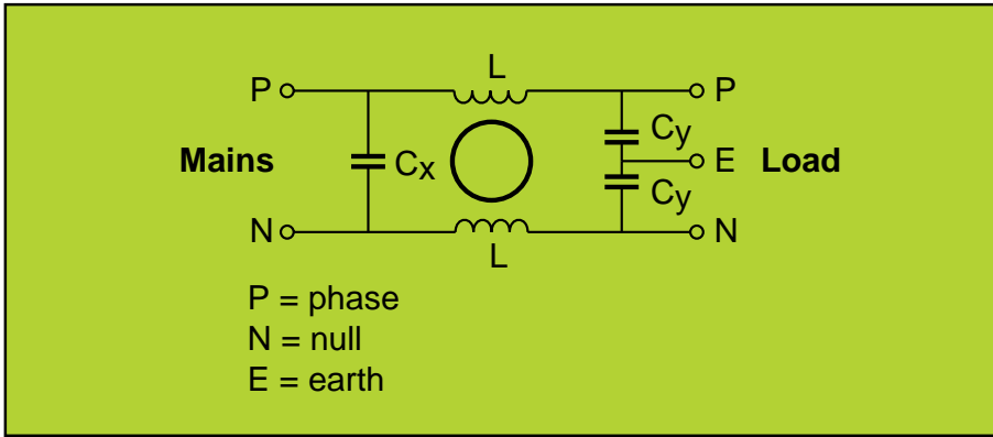
Fig. 8 Typical mains filter configuration.
