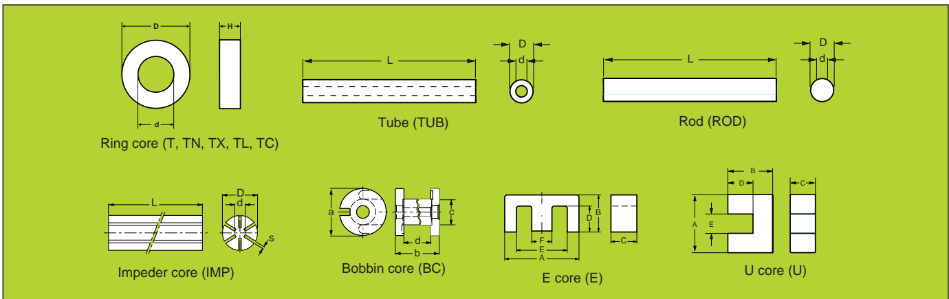
Fig. 9 Some products used in power applications.
