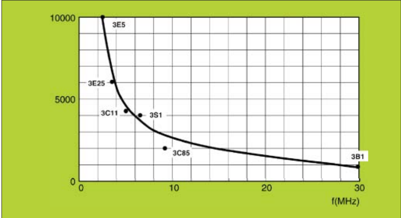
Fig. 4 Frequency of impedance peak for some MnZn ferrite materials.
