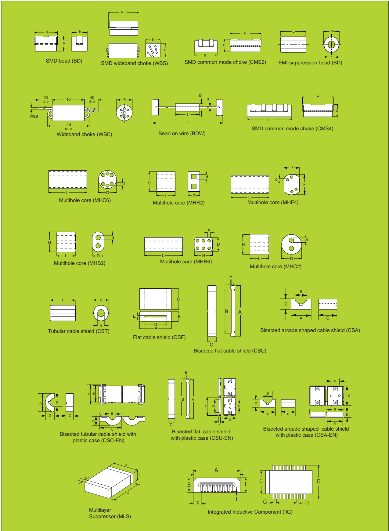
Fig. 7 Overview of small signal suppression products
