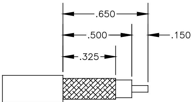
STRIPPING DIMENSIONS
